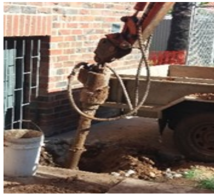
Underpinning Preparation
